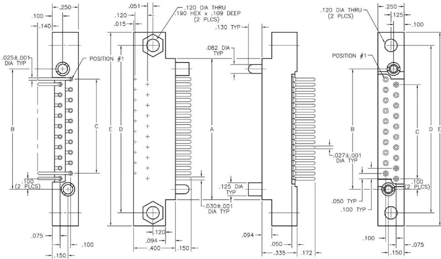
PLUG
