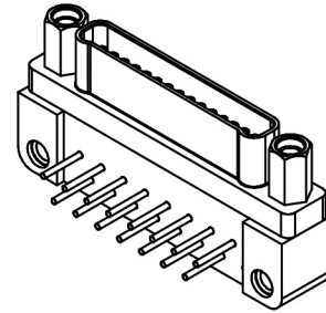
MK-162-015-435-220S (RECEPTACLE)
