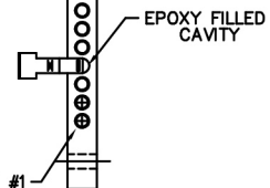
TERMINATION VIEW
