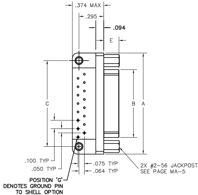
PLUG SHOWN
