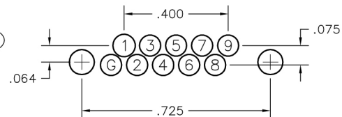
9 POSITION
